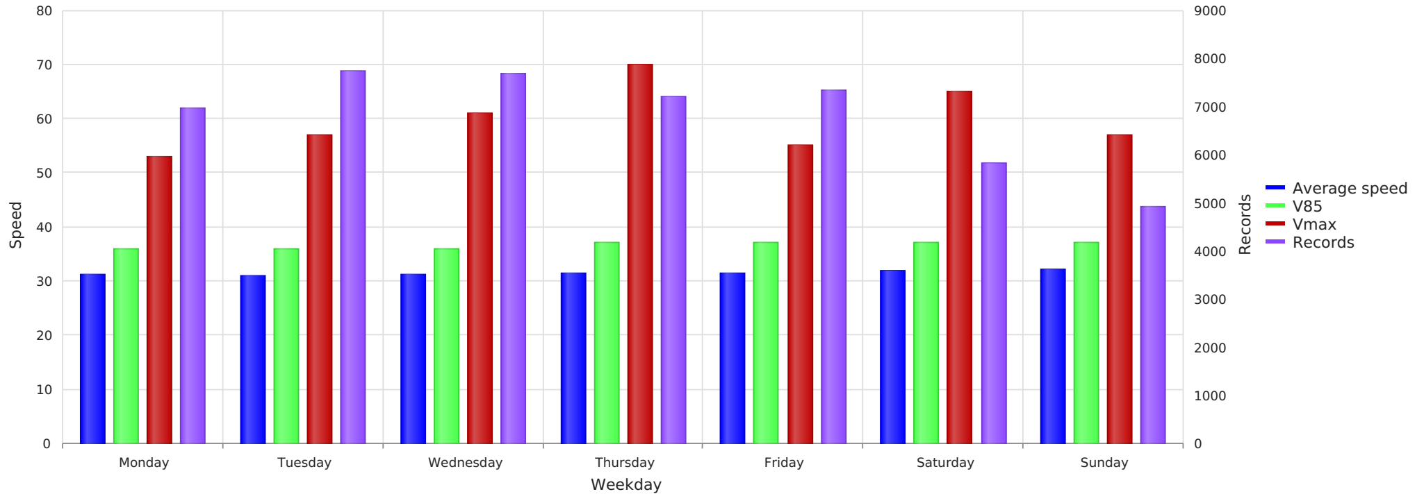
The Street Village Hall Eastbound 30 mph speed restriction Va, V85, Vmax Number of records vs. Weekday
